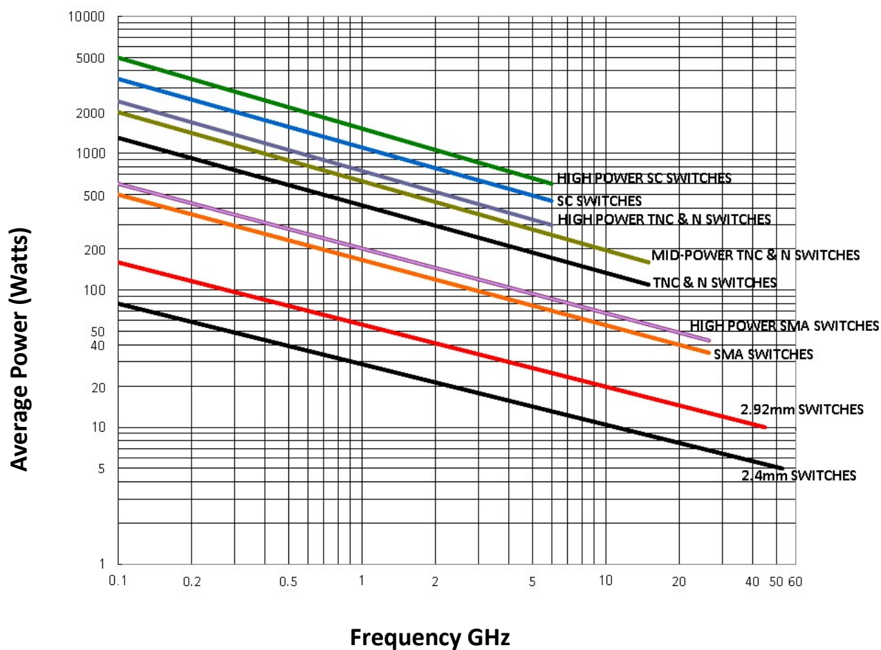
POWER HANDLING vs. FREQUENCY
